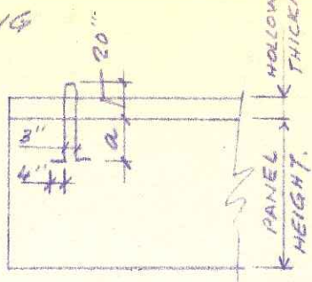
PANEL WITH LEDGE (EXTERIOR JOINT).
