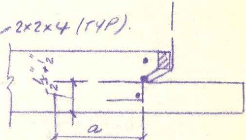
PANEL WITH LEDGE.
