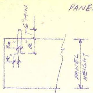
BEARING PANEL (TYP. BUTT JOINT).
