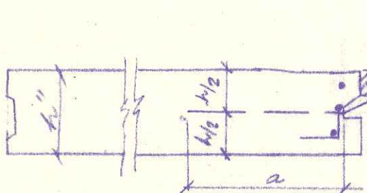
PANEL WITHOUT LEDGE
